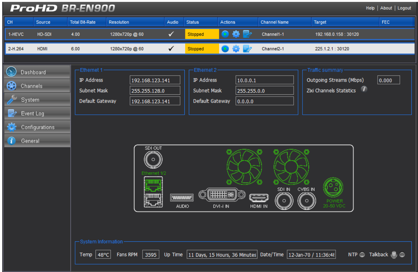
Figure 4-2: The Dashboard page
